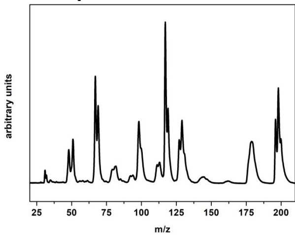
Mass spectrum
