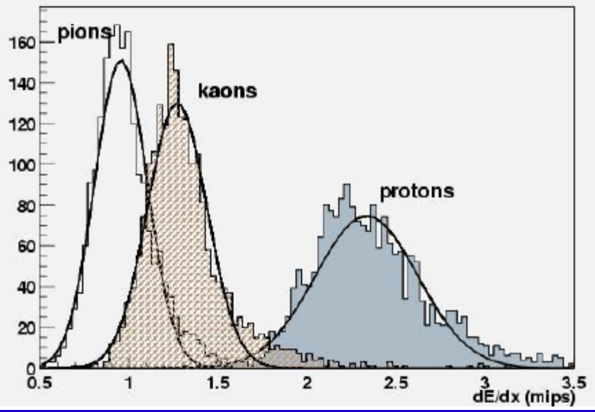
Momentum 730-830 MeV/c
