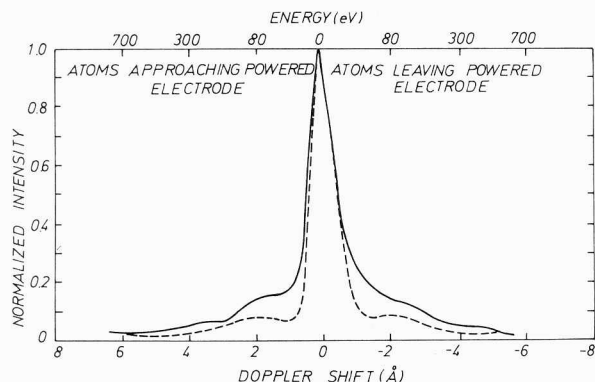
Fig. 4. Balmer \beta Doppler profiles observed in 200 kHz discharge in H_2 at two different pressures; 0.3 Torr (solid curve) and 0.55 Torr (dashed curve).
