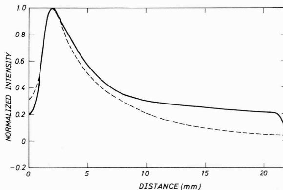
Fig. 1. Spatial profile of Balmer \beta radiation in 100 kHz discharge at p=0.65 Torr; peak radiation (solid curve); wing radiation (dashed curve).
