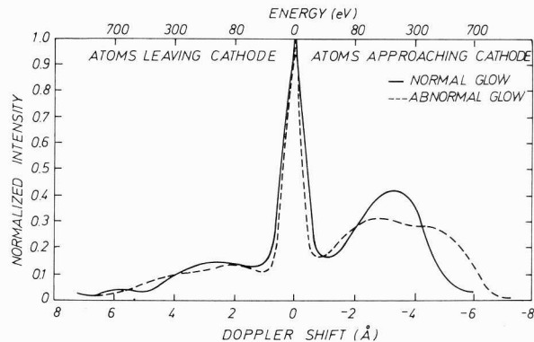
Fig. 5. Balmer \beta Doppler shift observed in hydrogen dc normal and abnormal glow discharge at the same pressure p=0.65 Torr. (—) I=2 mA, U=510 V; (---) I=10 mA, U=856 V.
