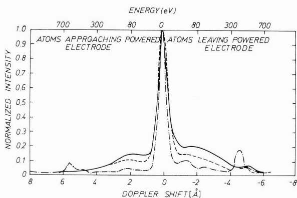
Fig. 2. Balmer \beta Doppler shift observed in rf glow discharge in H_2 at different frequencies at the same pressure p=0.55 Torr; 50 kHz (solid curve); 300 kHz (dashed curve); 13.56 MHz (chain curve).
