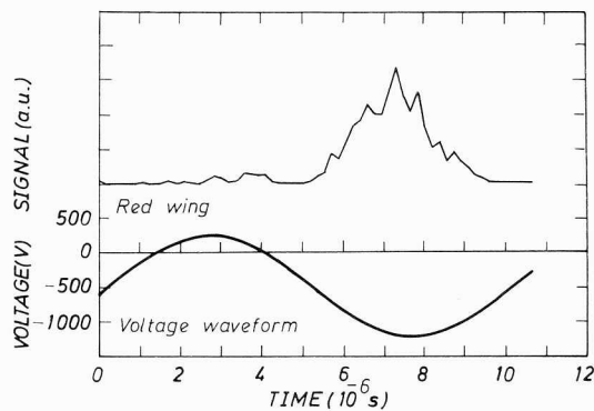
Fig. 3. Time-resolved emission profile of Balmer \beta red wing \lambda=4863 Å, together with the voltage waveform in 100 kHz discharge at p=0.65 Torr.
